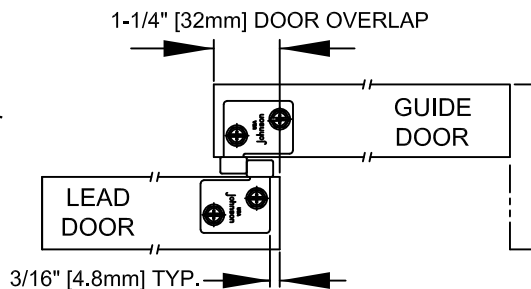
VIEW OF 2054 MULTI-DOOR PULL CATCH
