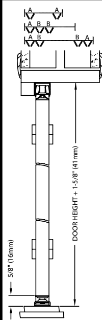
1725AOSB Components
