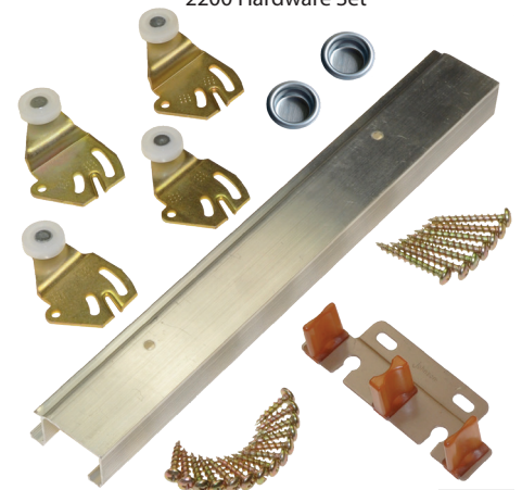
2200 Hardware Set
